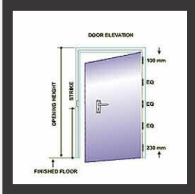
Insulated Metal Doors
